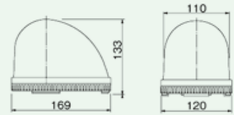
32-393 RWM-24 (黄) 32-394 RWM-24 (青)
