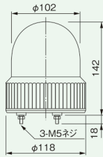
32-397 SKHE-100 (黄) 32-398 SKHE-100 (赤)
